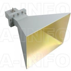
LB-340-15-C-SF Standard Gain Horn Antenna 2.2-3.3GHz 15dB Gain SMA Female
