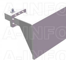
LB-340-15-C-NFSPO Standard Gain Horn Antenna 2.2-3.3GHz 15dB Gain N Type Female
